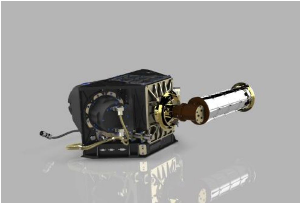
Instrument PHEBUS
